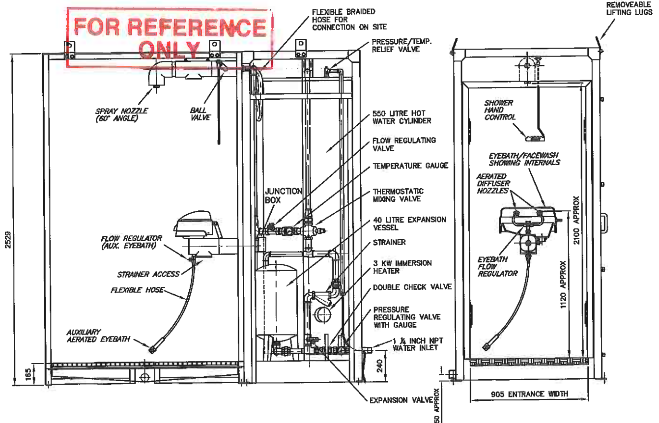
SIDE VIEW - SIDE/DOOR PANNELLING & INSULATION OMMITED TO SHOW INTERNALS
